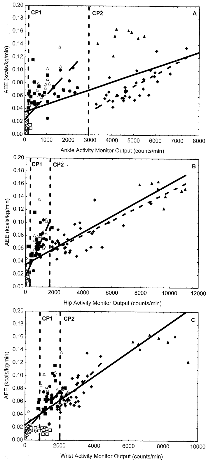
Figure 1. Single and double regression modeling strategies for predicting activity energy expenditure (AEE, \text{kcal}\cdot\text{kg}^{-1}\cdot\text{min}^{-1} ) from Actical® activity monitor output at the ankle (A), hip (B), and wrist (C) during nine activities ( n = 24 children): hand writing (open circles), card sorting with hands (open squares), video game playing (open diamonds), floor sweeping (open triangles), carpet vacuuming (closed circles), table dusting (closed squares), treadmill and overground walking (closed diamonds), and treadmill jogging (closed triangles). The first vertical dashed line is the cut point (CP1) between sitting activities and cleaning activities, while the second vertical dashed line is the cut point (CP2) between cleaning and locomotion activities. Best fit regression lines shown include the following: (a) solid line for 1R model, (b) long dashed for sitting and cleaning activities in 2R model, and (c) dotted line for locomotion activities in 2R model (line was fit for walking activities only for ankle monitor output).
