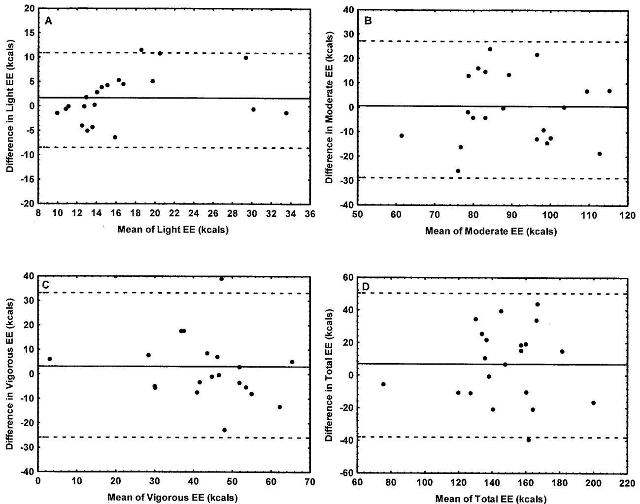
Figure 6. Bland-Altman plots for hip activity monitor (double regression modeling hip algorithm with 1-min bouts) showing difference scores (actual-predicted) in activity energy expenditure (AEE) plotted against the average of actual and predicted values for light (A), moderate (B), vigorous (C), and total AEE (D). Solid line = mean of the difference scores; dashed lines = 95% confidence interval for difference scores.
