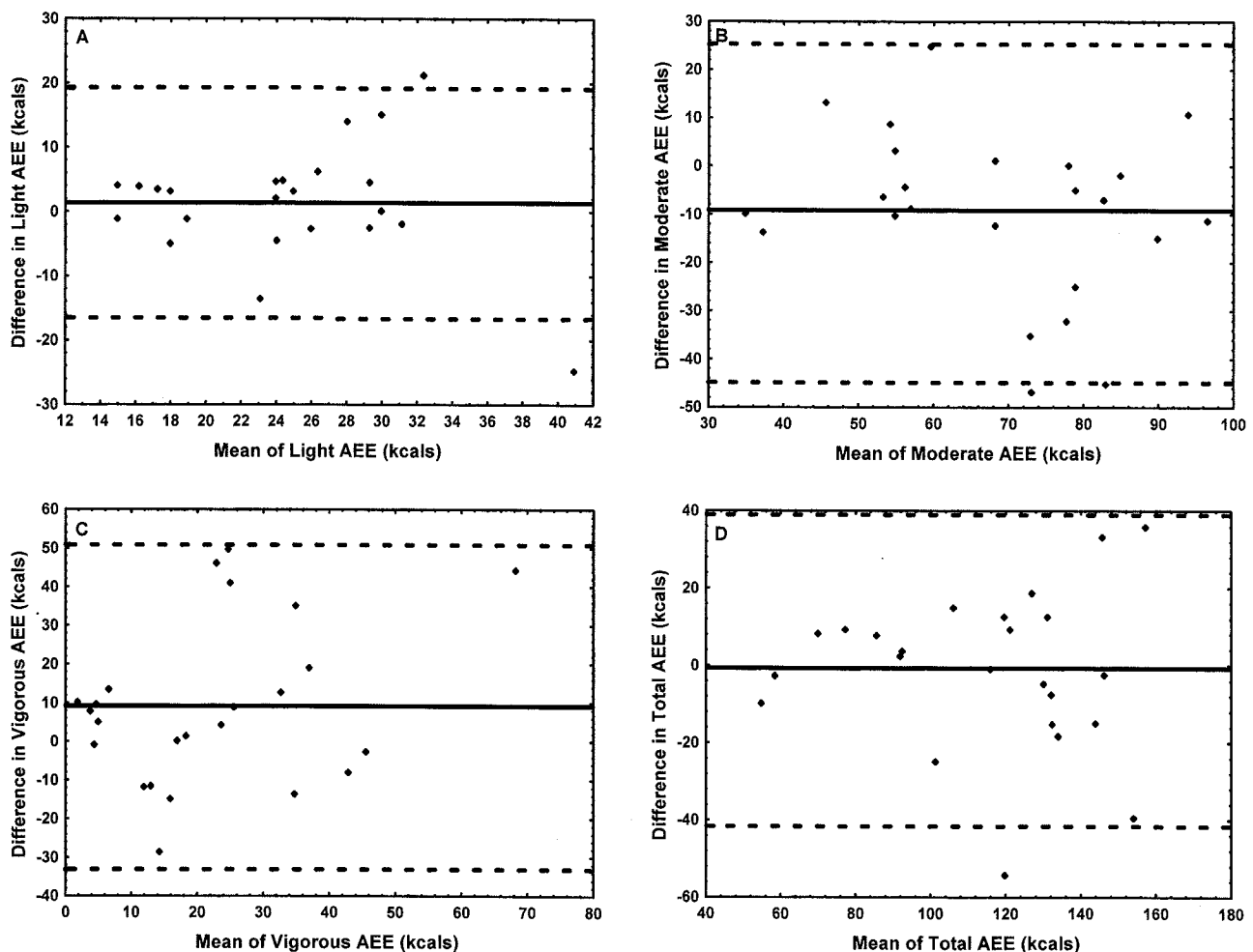
Figure 4. Bland-Altman plots for hip activity monitor (double regression modeling hip algorithm with 1-min bouts) in children showing difference scores (actual-predicted) in activity energy expenditure (AEE) plotted against the average of actual and predicted values for light (A), moderate (B), vigorous (C), and total AEE (D). Solid line = mean of the difference scores; dashed lines = 95% confidence interval for difference scores.
