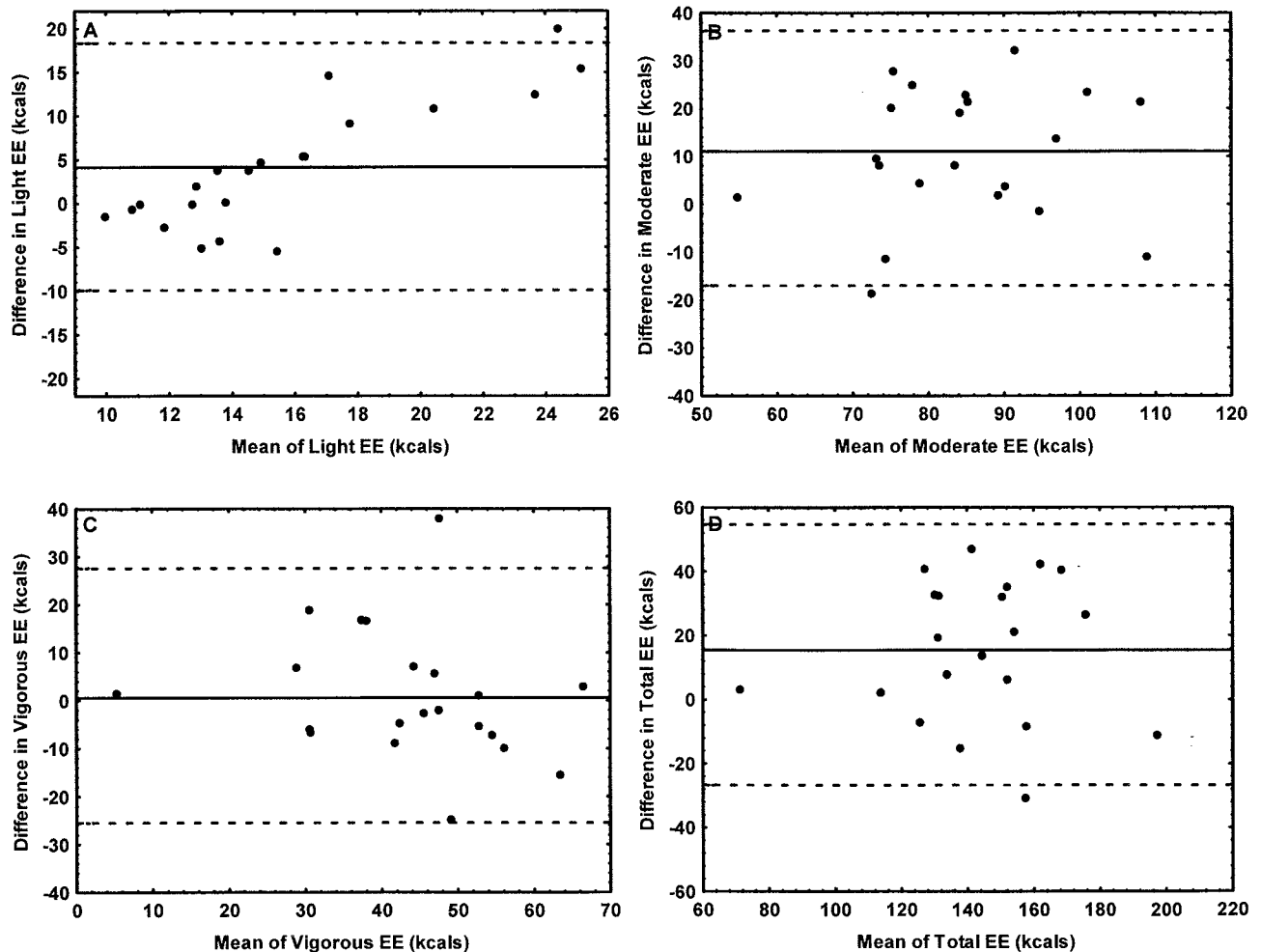
Figure 5. Bland-Altman plots for hip activity monitor (single regression modeling hip algorithm with 1-min bouts) showing difference scores (actual-predicted) in activity energy expenditure (AEE) plotted against the average of actual and predicted values for light (A), moderate (B), vigorous (C), and total AEE (D). Solid line = mean of the difference scores; dashed lines = 95% confidence interval for difference scores.
