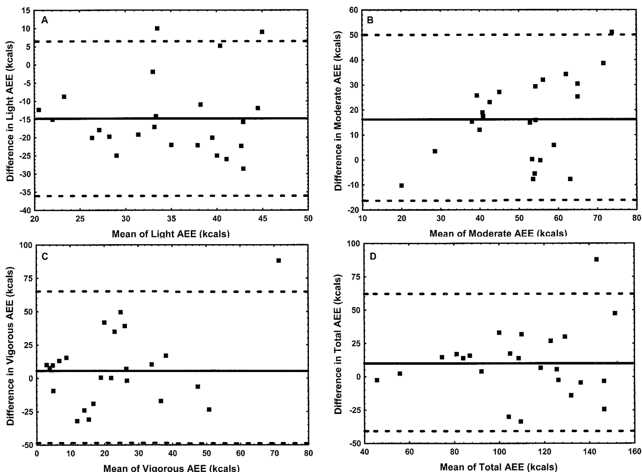
Figure 3. Bland-Altman plots for hip activity monitor (single regression modeling hip algorithm with 1-min bouts) in children showing difference scores (actual-predicted) in activity energy expenditure (AEE) plotted against the average of actual and predicted values for light (A), moderate (B), vigorous (C), and total AEE (D). Solid line = mean of the difference scores; dashed lines = 95% confidence interval for difference scores.
