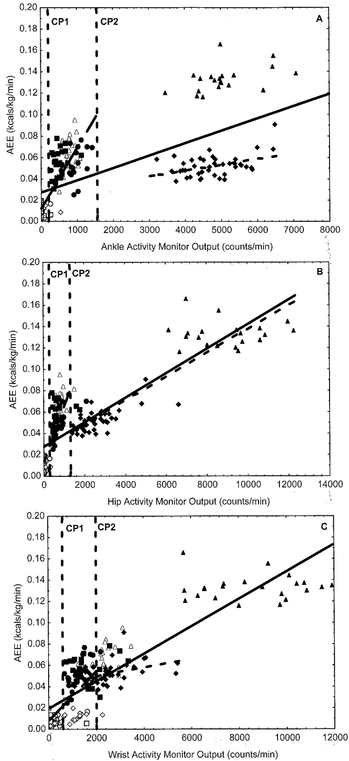
Figure 2. Single and double regression modeling strategies for predicting activity energy expenditure (AEE, \text{kcal}\cdot\text{kg}^{-1}\cdot\text{min}^{-1} ) from Actical® activity monitor output at the ankle (A), hip (B), and wrist (C) during nine activities ( n = 24 adults): typing (open circles), hand writing (open squares), card sorting with hands (open diamonds), floor sweeping (open triangles), carpet vacuuming (closed circles), table dusting (closed squares), treadmill walking (closed diamonds), and treadmill jogging (closed triangles). The first vertical dashed line is the cut point (CP1) between sitting activities and cleaning activities, while the second vertical dashed line is the cut point (CP2) between cleaning and locomotion activities. Best fit regression lines shown include the following: (a) solid line for 1R model, (b) long dashed for sitting and cleaning activities in 2R model, and (c) dotted line for 2R locomotion activities (walking only for ankle and wrist output).
